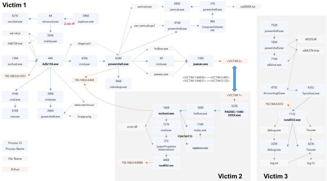
Fig. 14. Provenance Graph of FIN7 Scenario
