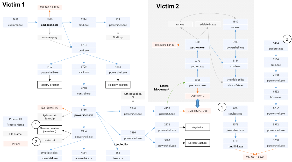
Fig. 13. Provenance Graph of APT29 Scenario
